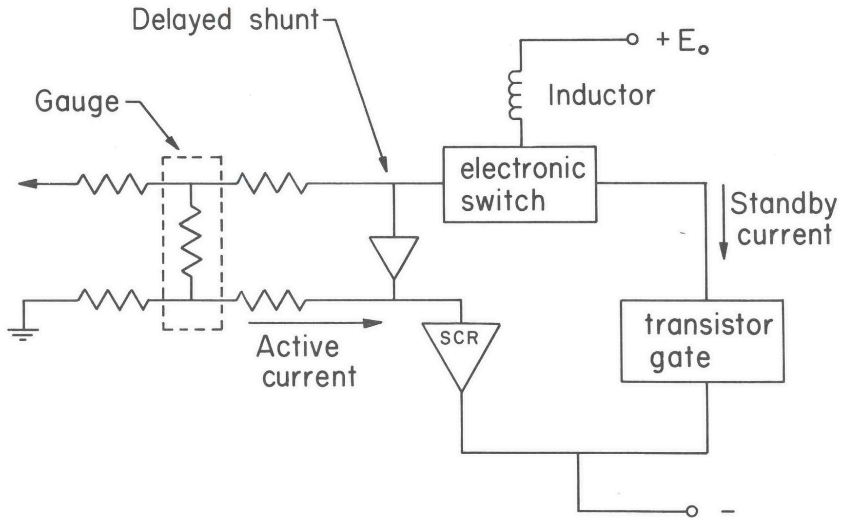
Fig. 21. Block diagram of constant current supply for use with manganin gauges.
